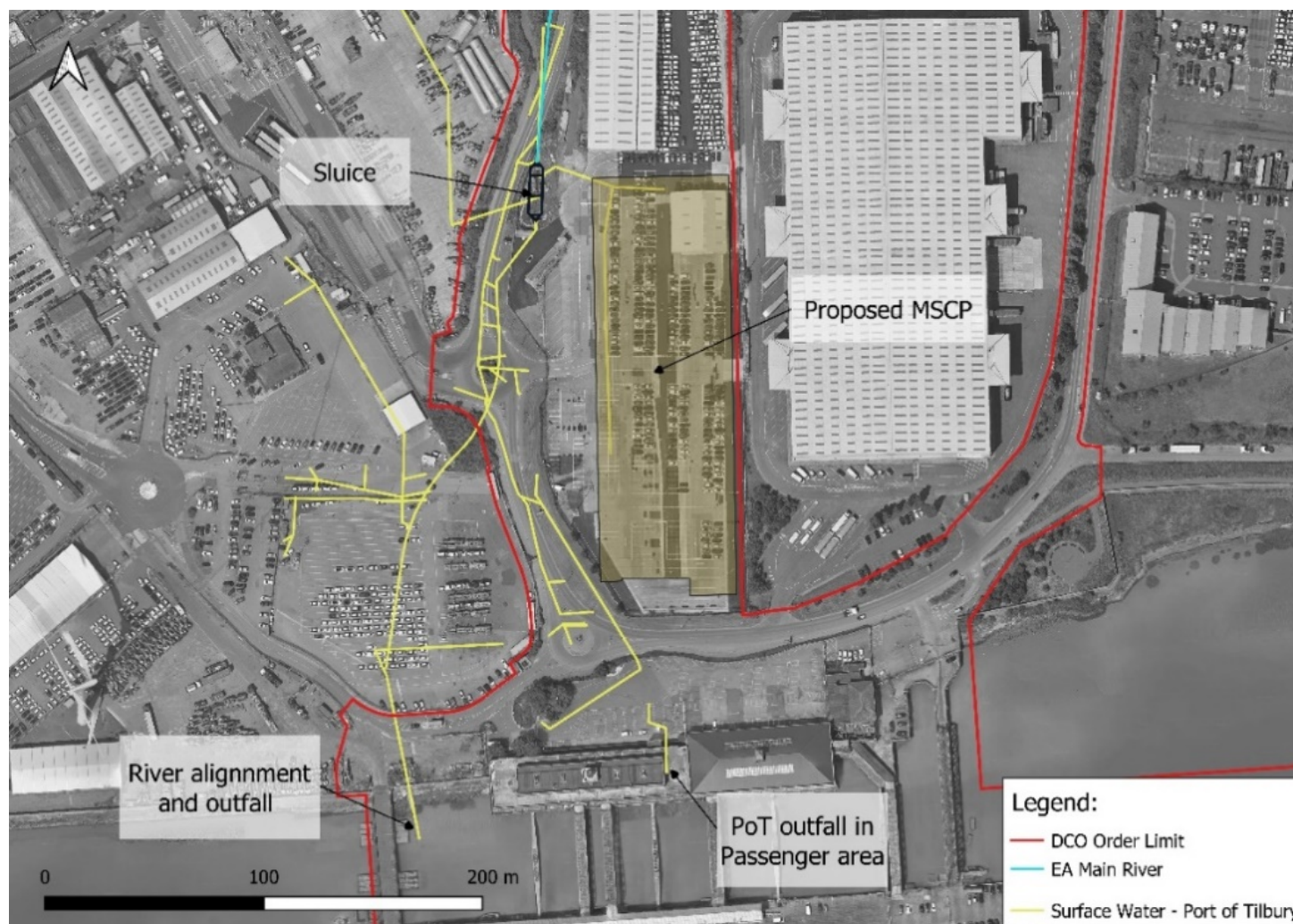
Figure 17.11: Existing drainage pipes and EA main rivers around the site.
